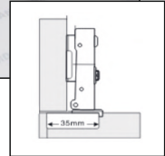
Balama semiaplicata fara arc Push Open
